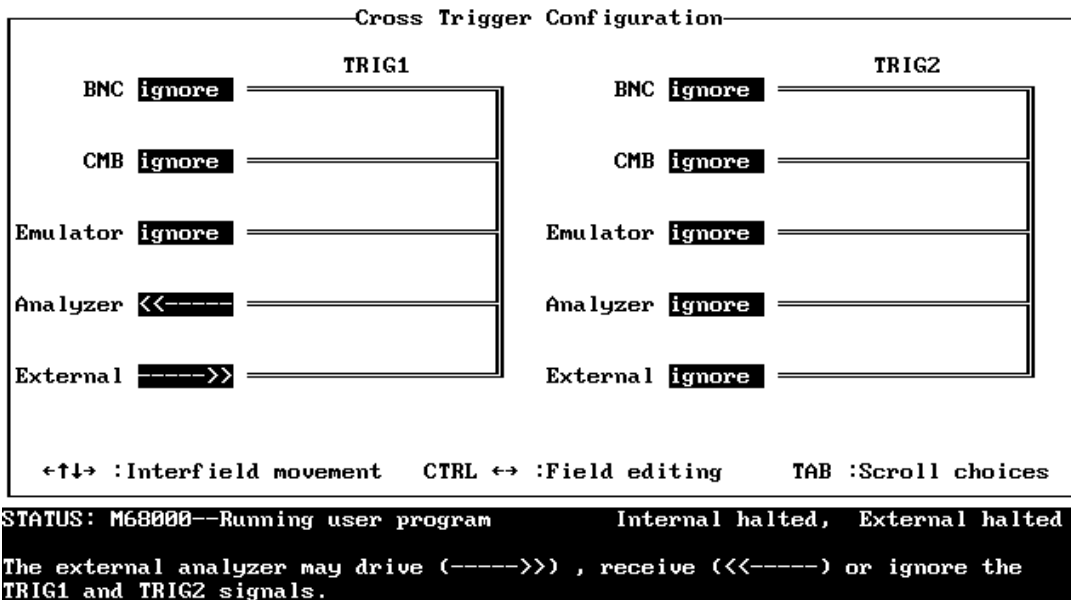
Figure 6-3. Using One Analyzer to Arm the Other
